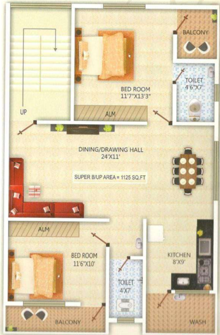
Typical 1st To 3rd Floor Plan
